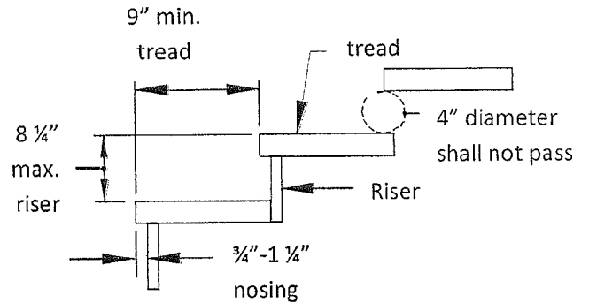
Figure 22. Treads and Risers
