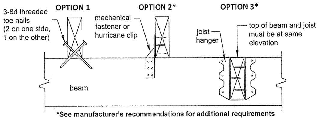
Figure 5. Joist-to-Beam Detail
